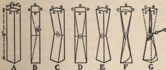
FIG. 44.—How to Prepare a 9-inch Propeller.
